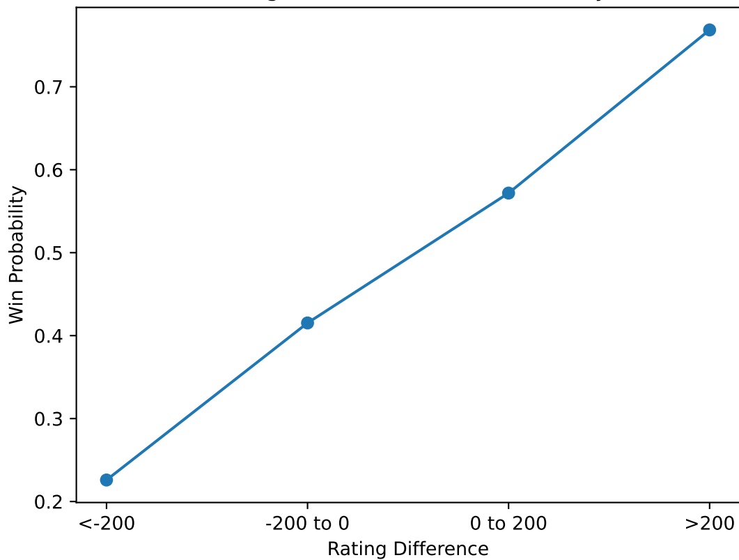
Rating Difference vs Win Probability
